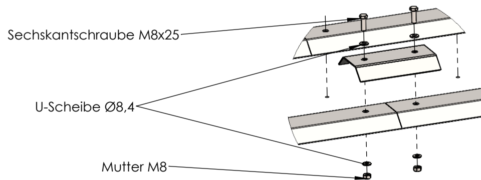
DETAIL B
